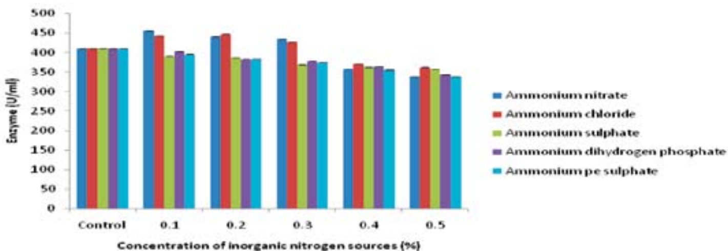
Fig. 3 : Effect of different concentration of inorganic nitrogen sources on production of enzyme ANOVA of different inorganic nitrogen sources; Ammonium nitrate- F= 1.74 , p < 0.000 ; Ammonium chloride- F= 1.34 , p < 0.000 ; Ammonium sulphate- F= 3.56 , p < 0.000 ; Ammonium dihydrogen phosphate- F= 6.47 , p < 0.000 ; Ammonium pe sulphate- F= 6.05 , p < 0.000 . Means of each inorganic nitrogen sources checked for significant at 5% level.
